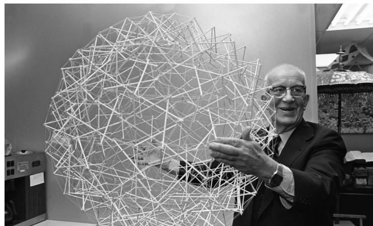
Fig. 5. Tensegrity Sphere by Buckminster Fuller.
