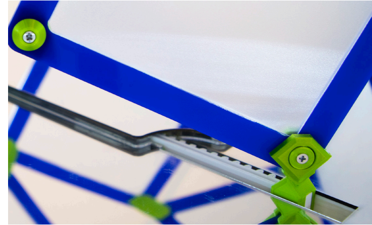
Fig. 45. A close-up of the joint that connects the model to the rack.
