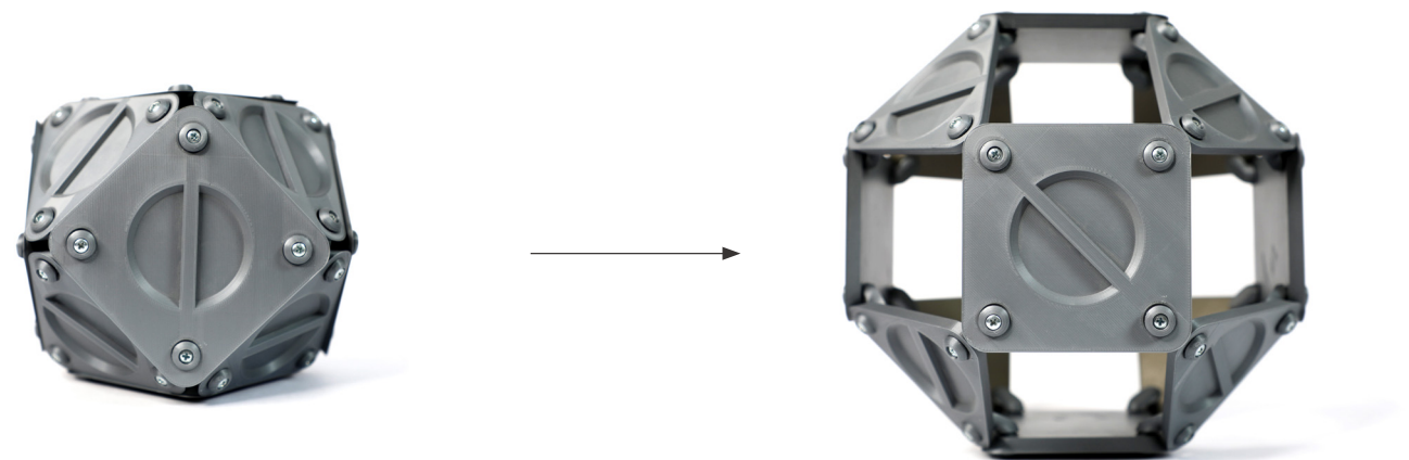
Fig 34. An octahedron that transforms into a cuboctahedron.
